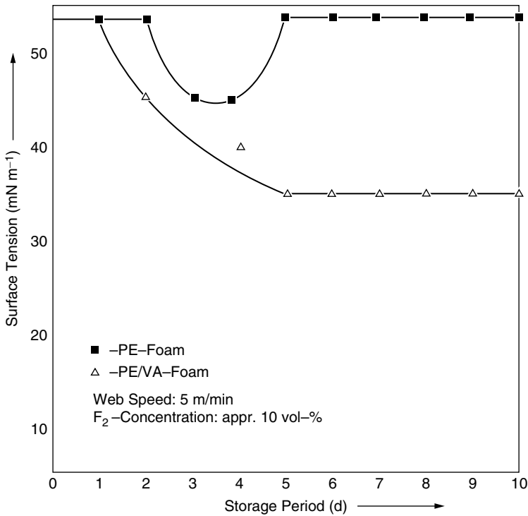
FIGURE 40.3 Storage stability of the surface energy of polyethylene (PE) and PE–vinyl acetate (VA) copolymer foams subjected to fluorine pretreatment.
