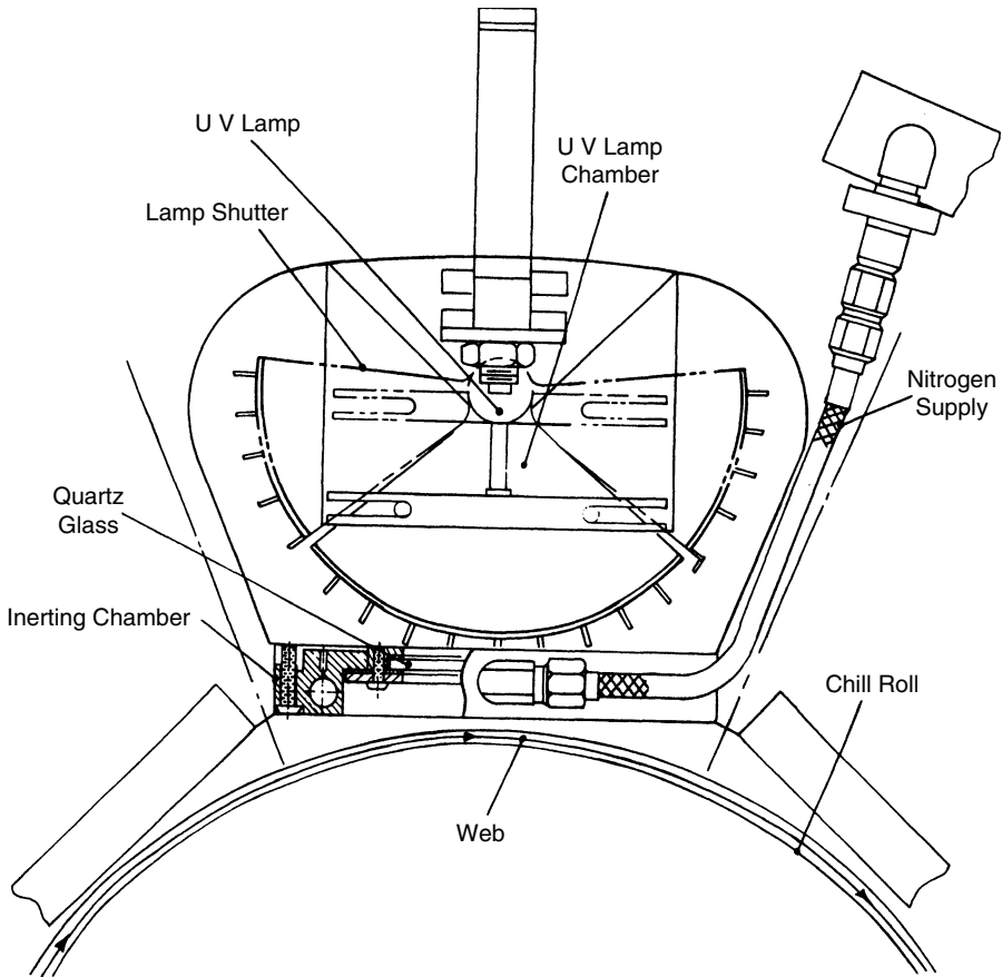
FIGURE 21.1 UV irradiation with nitrogen inverting.
