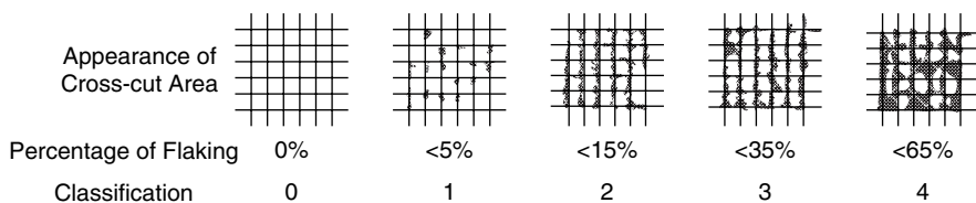
FIGURE 6.3 Principle of classifying paint film adhesion in the cross-cut test.
