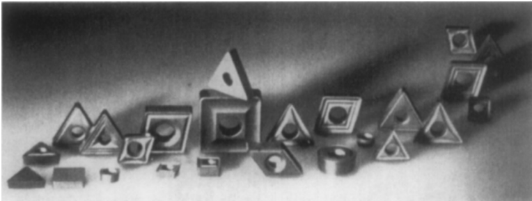
FIGURE 35.5 Photography showing cemented tungsten carbide cutting tool inserts coated with TiC and TiN coating in a conventional CVD process. These coatings impart improved wear resistance to the carbide tools, allowing them to run at higher speeds and chip loads in the machining of various materials.
