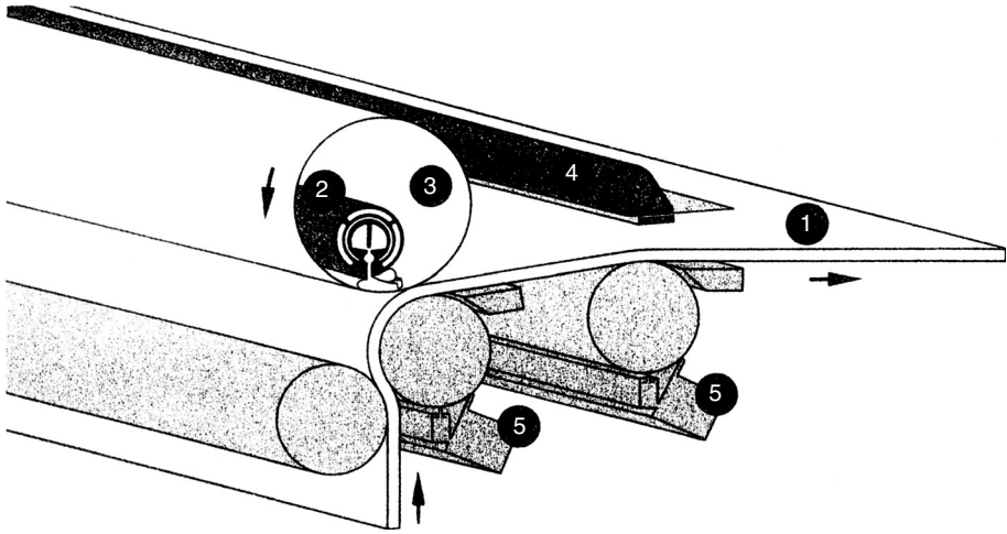
FIGURE 22.2 Foam coater. 1: web; 2: squeegee; 3: screen; 4: whisper blade; 5: doctor blade.
