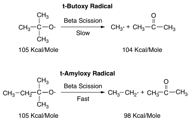
FIGURE 73.1 The \beta -scission reactions.
