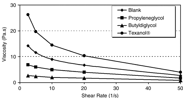
FIGURE 85.5 Influence of cosolvents and coalescents on the viscosity developed by a PEUPU thickener. In each case, 3% cosolvent was added to the pure acrylic latex.
