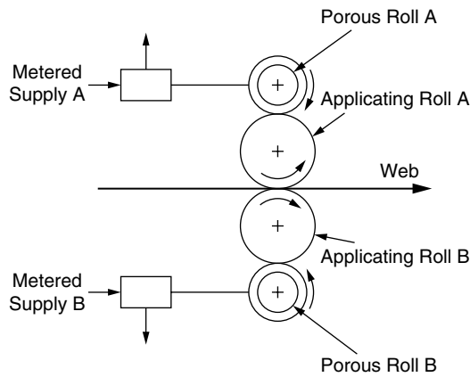
FIGURE 21.12 Two-side coating with porous rolls.
