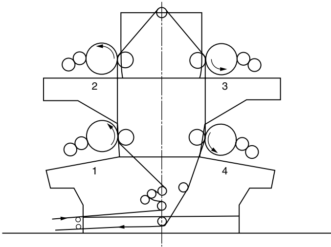
FIGURE 24.1 Flexo end printer with four color decks.
