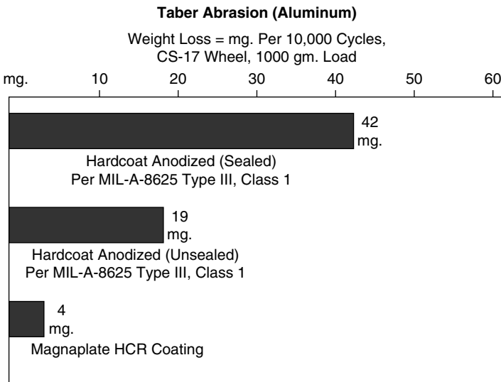
FIGURE 34.4 Weight loss following Taber abrasion for aluminum samples with various coatings.
