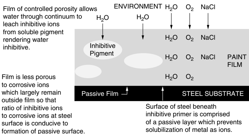
FIGURE 102.5 Corrosion protection by inhibitive primer.
