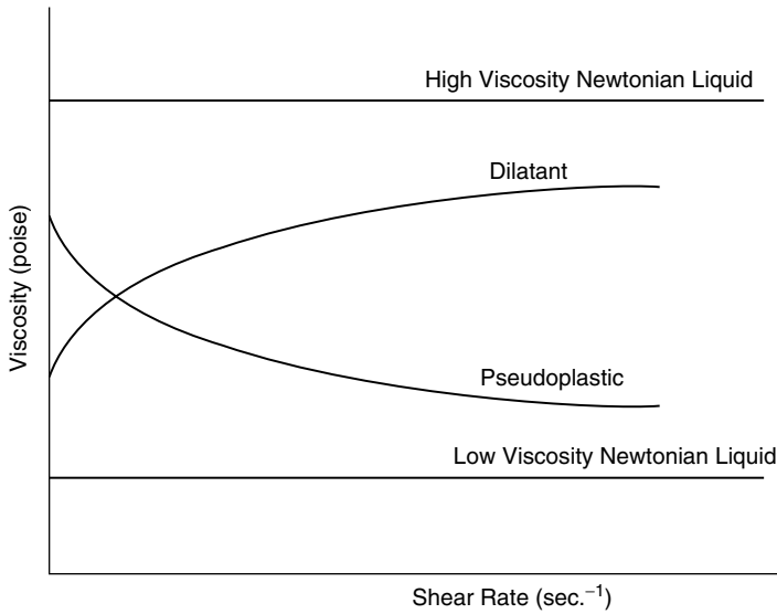
FIGURE 1.2 Viscosity shear rate curves.
