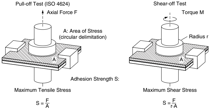
FIGURE 6.4 Methods for quantitative determination of adhesion strength.
