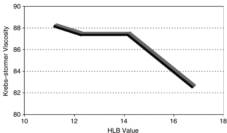
FIGURE 85.6 Influence of dispersant HLB value on the mid-shear viscosity developed by a PEUPU thickener in a standard latex paint. (After Rheology Handbook: A Practical Guide to Rheological Additives , Hightstown, NJ: Elementis, Inc., 2000.)
