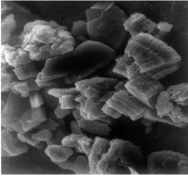
FIGURE 82.1 Hydrous kaolin. (From Engelhard Corp. technical literature.)
