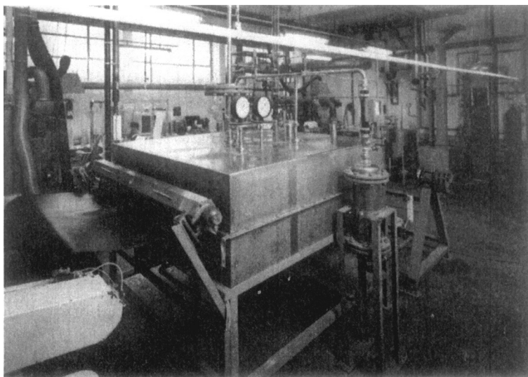
FIGURE 40.2 The surface fluorination pilot plant of Lohmann GmbH, Neuweid, Germany.
