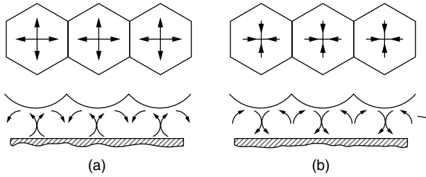
FIGURE 2.11 Schematic illustration of the formation of the Bernard cells due to (a) the surface tension gradient and (b) the density gradient.
