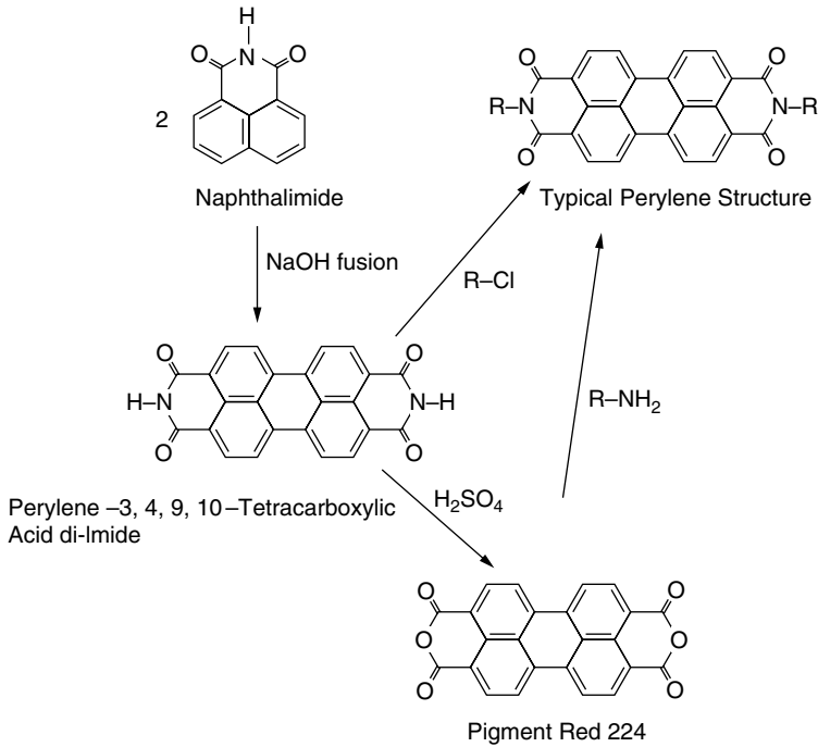
FIGURE 78.13 Perylene synthesis.
