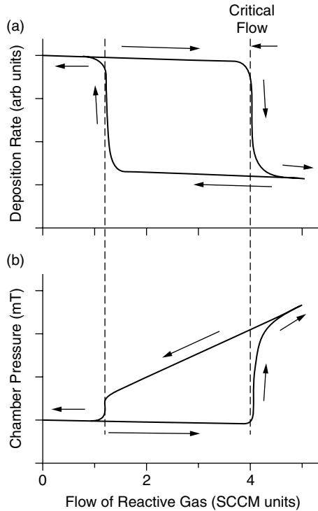
FIGURE 31.8 Hysteresis curves for the deposition rate (a) and the chamber pressure (b) for the case of reactive sputtering.
