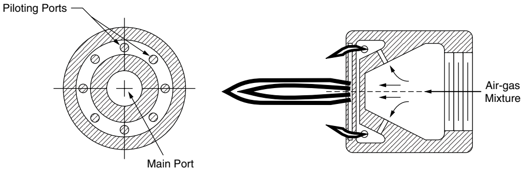
FIGURE 38.3 Gun-type nozzles.
