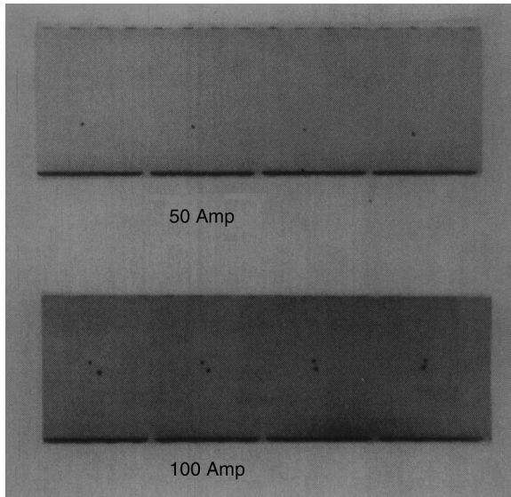
FIGURE 32.2 Number of arc spots on the titanium cathode arc source as a function of arc current.
